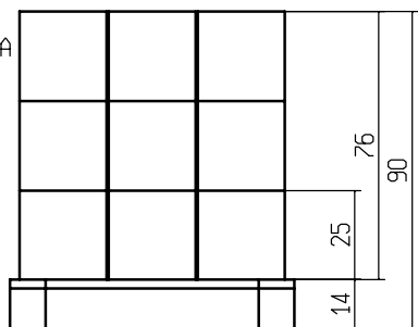
MAX 36 SCATOLE PICCOLE MAX 36 SMALL BOXES
